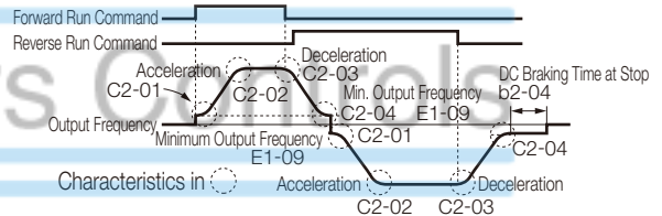
Time Chart when Switching Forward Run and Reverse Run at Deceleration to Stop (V/f control mode example)
