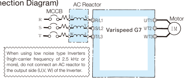
(Connection Diagram)
