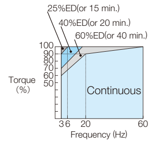
Allowable Load Characteristics of Yaskawa's Standard Motor
