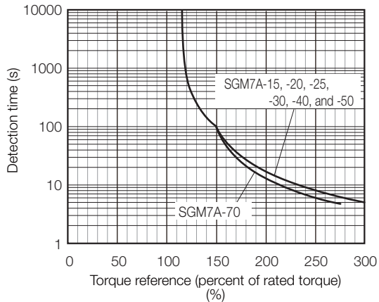
SGM7A-15, -20, -25, -30, -40, -50, and -70
