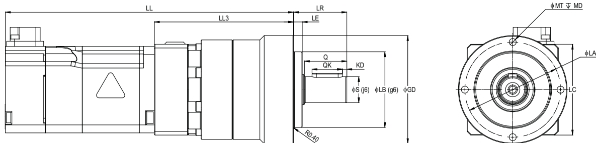
Shaft Detail (VL050 Models Only)
