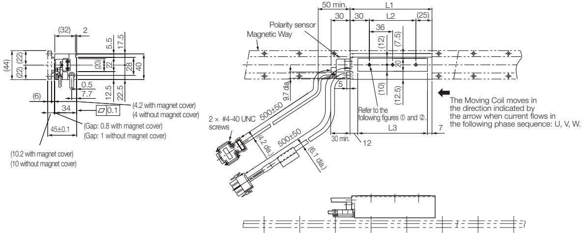
① SGLFW-20A090A□
