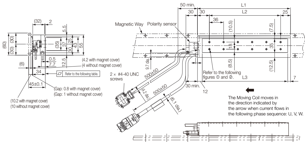
① SGLFW-35A120A□D
