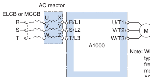
Connection Diagram
