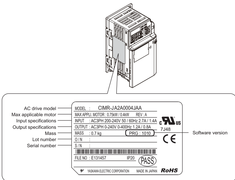
Figure 1 Nameplate Information
